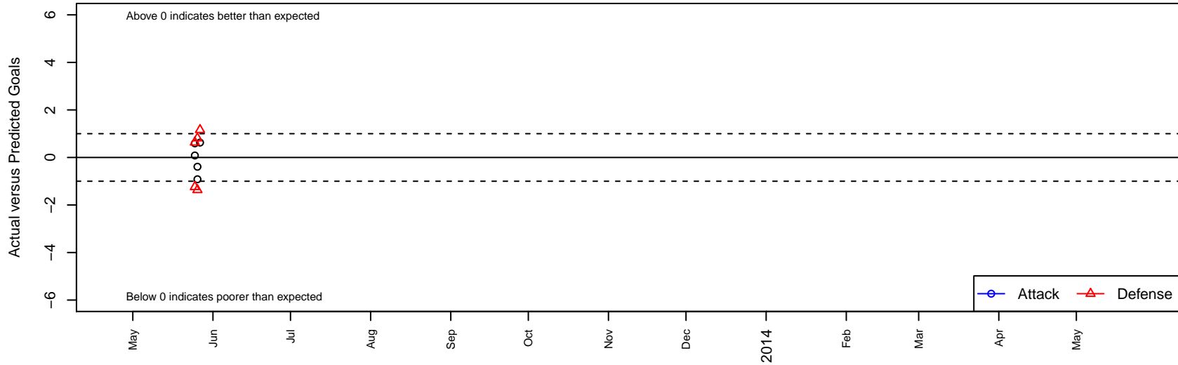
Sagebrush Sparks Freedom G01 Dots are actual minus expected GF (blue circles) and GA (red triangles). Blue line is smoothed change in attack strength. Red is smoothed change in defense strength.
